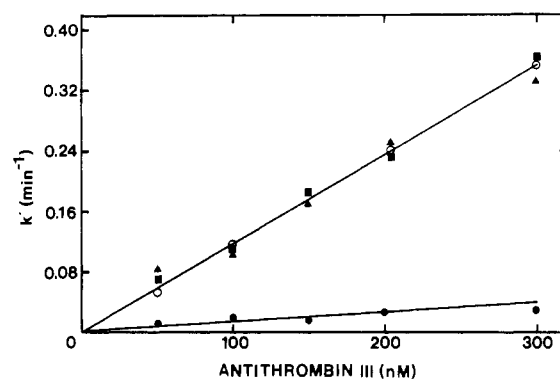
FIGURE 5: Pseudo-first-order rate constant of inhibition of factor X_a as a function of antithrombin III concentration. Prothrombin was activated by ( \bullet ) factor X_a /factor V_a /phospholipid/ Ca^{2+} , ( \circ ) factor X_a /factor V_a / Ca^{2+} , and ( \blacktriangle ) factor X_a /phospholipid/ Ca^{2+} . The concentrations of the various reaction components are listed in Table I, rows 1, 2, and 3, respectively. The pseudo-first-order rate constant of inhibition of factor X_a was determined as described in Figure 3. The pseudo-first-order rate constants of inhibition of free factor X_a ( \blacksquare ) were determined as described under Materials and Methods.
