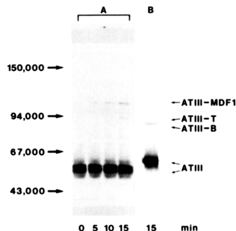
FIGURE 9: Identification of molecular species with thrombin activity in the prothrombin activation mixture. Prothrombin (1.0 \mu\text{M} ) was activated by 3 pM factor X_a /0.1 nM factor V_a /10 \mu\text{M} phospholipid/5 mM \text{CaCl}_2 . Samples were removed at the times indicated, incubated with antithrombin III (1 \mu\text{M} ) and heparin (1 \mu\text{g/mL} ), and subjected to sodium dodecyl sulfate gel electrophoresis. (A) Unreduced samples; (B) disulfide-reduced sample. Abbreviations: ATIII, antithrombin III; MDF1, meizothrombin (des fragment 1); T, \alpha -thrombin; B, B chain of \alpha -thrombin. Experimental details are given under Materials and Methods.
