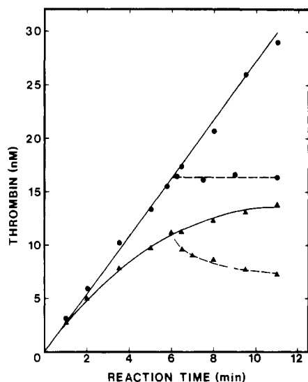
FIGURE 1: Inhibition of thrombin formation and thrombin activity in prothrombin activation mixtures by antithrombin III. Prothrombin (0.5 μM) was activated by factor X a (4.0 nM)/phospholipid (5 μM)/CaCl 2 (10 mM) either in the absence (●) or in the presence (▲) of 100 nM antithrombin III. At timed intervals, samples were taken and assayed for thrombin activity. In separate experiments, soybean trypsin inhibitor (20 μg/mL) was added 6 min after starting the reaction with factor X a . The time courses of thrombin activity are indicated by the dashed lines.
