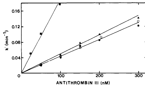
FIGURE 4: Pseudo-first-order rate constant of inhibition of thrombin activity as a function of antithrombin III concentration. Prothrombin was activated by ( \bullet ) factor X_a /factor V_a /phospholipid/ Ca^{2+} , ( \circ ) factor X_a /factor V_a / Ca^{2+} , and ( \blacktriangle ) factor X_a /phospholipid/ Ca^{2+} . The concentrations of the reactants are listed in Table I, rows 1, 2, and 3, respectively. Antithrombin III was present at various concentrations. The pseudo-first-order rate constants of inhibition of thrombin activity were determined as described in Figure 2. The pseudo-first-order rate constant of inhibition of \alpha -thrombin ( \blacksquare ) was determined as described under Materials and Methods.
